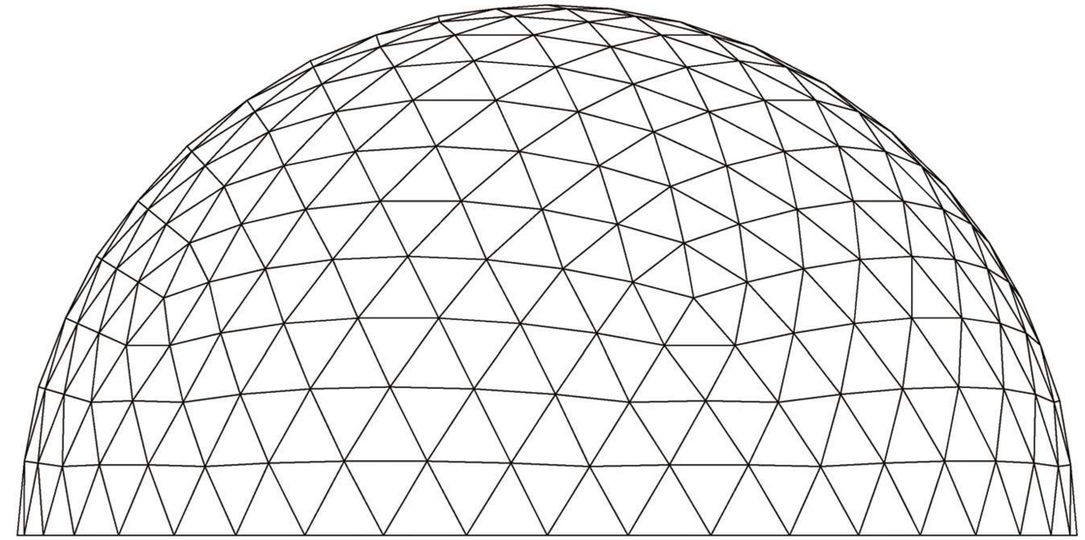
FREQUENCY 8
