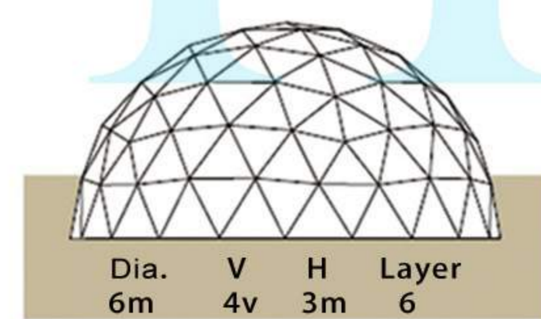
Geodesic Dome
